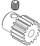
500405611 Piniongear Motorritzel
